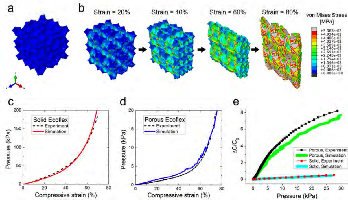
Figure 3. FE simulations to investigate the compressive behavior of solid and microporous Ecoflex dielectric cubes. (a) A full 3-D representative model of the porous Ecoflex dielectric
